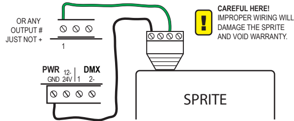
TRIGGERING FROM A SOLID-STATE OUTPUT (BOOBOX FLEX / FLEXMAX)
