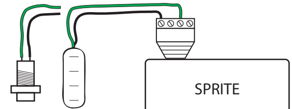
TRIGGERING FROM A BUTTON OR STEP MAT
