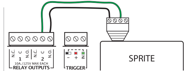
TRIGGERING FROM A RELAY OUTPUT (ALL PICOBOOS EXCEPT PICOBOO ONE)
